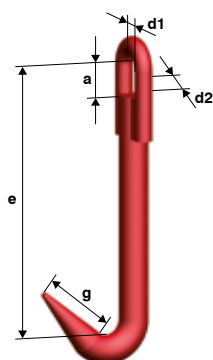
BA Ballenhaken
