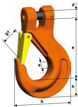
KHSW Kuppelhaken
